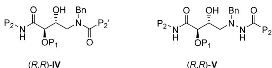
Figure 2. The reversed-statine based inhibitors presented in this report.
