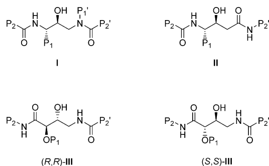
Figure 1. The structures of the hydroxyethylamine core ( I ) and the statine-derived core ( II ). ( R,R )- III and ( S,S )- III are reversed-statine based Plm inhibitors.
